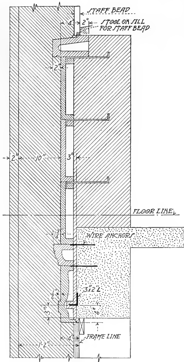
METHOD OF ANCHORING FACING TO BRICK SPANDREL WALLS
